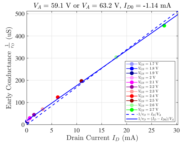
Figure 4.24: Early Conductance \frac{1}{r_O} vs. I_D
