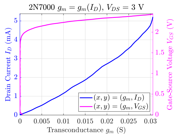
Figure 4.20: Transconductance g_m vs. I_D and V_{GS}
