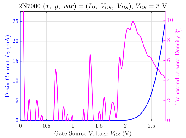
Figure 4.25: Transfer Characteristics I_D vs. V_{GS}
