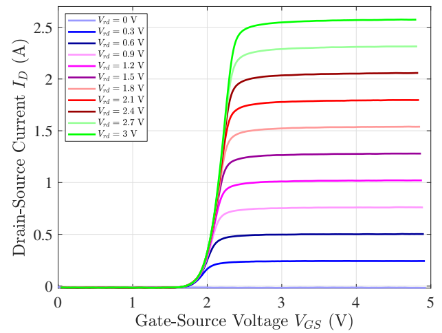
Figure 4.35: Transfer characteristics
