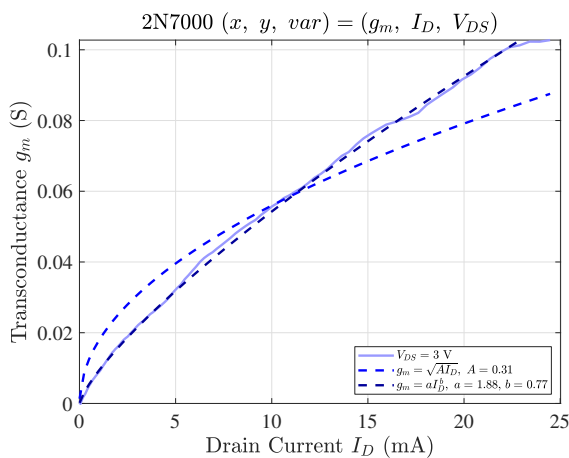
Figure 4.23: Transconductance g_m vs. I_D
