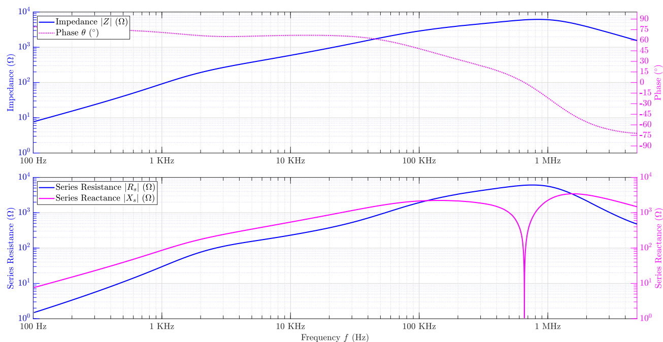
Figure 2.21: Impedance characteristics
