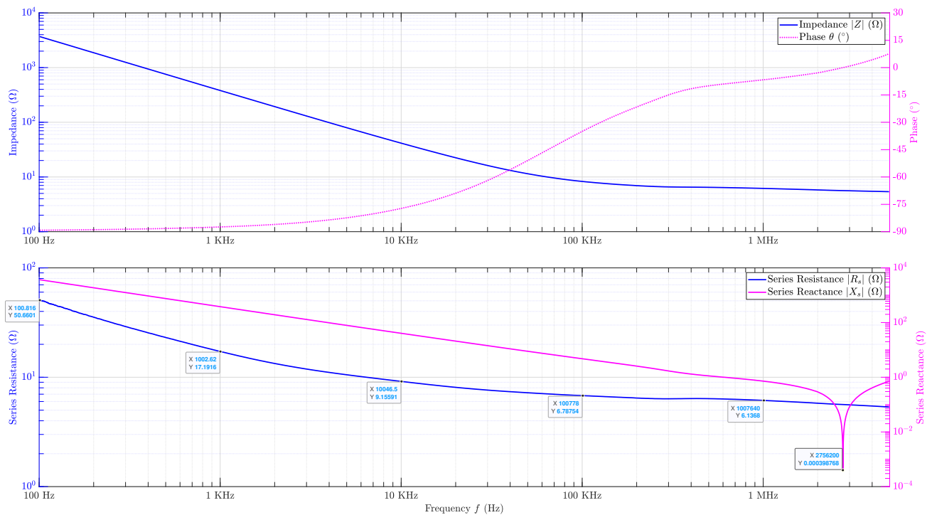
Figure 3.2: Impedance characteristics
