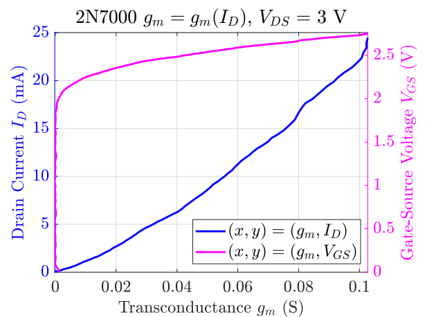
Figure 4.26: Transconductance g_m vs. I_D and V_{GS}
