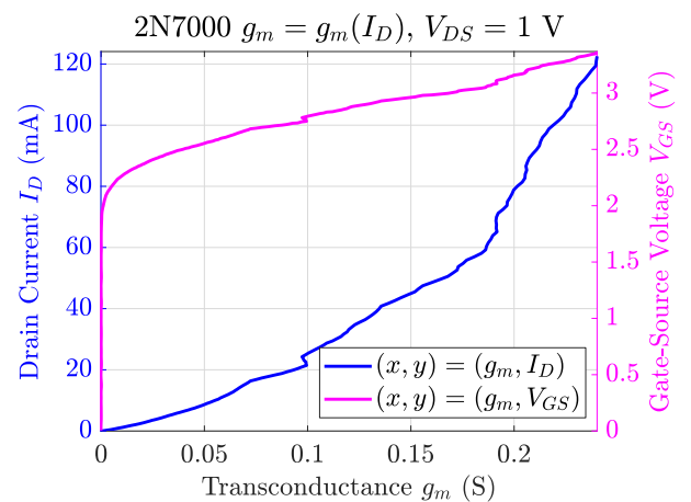
Figure 4.32: Transconductance g_m vs. I_D and V_{GS}
