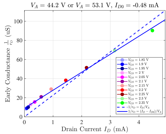
Figure 4.18: Early Conductance \frac{1}{r_O} vs. I_D
