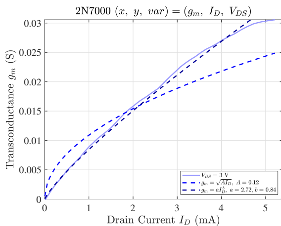
Figure 4.17: Transconductance g_m vs. I_D
