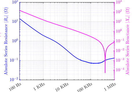
Figure 3.19: The capacitor's equivalent capacitance (left) and impedance characteristics (middle and right)
