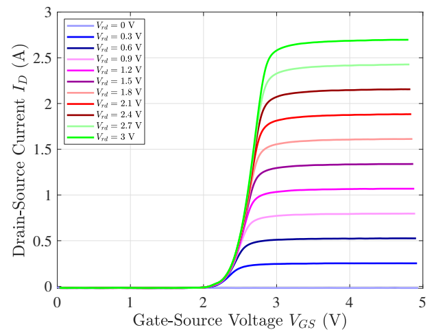
Figure 4.40: Transfer characteristics
