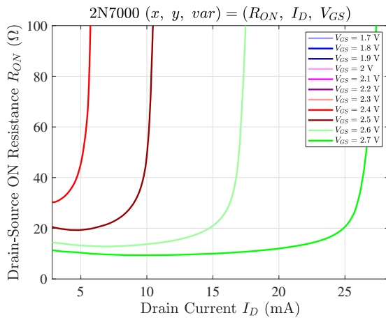
Figure 4.22: DS On-Resistance R_{DS(on)} vs. I_D
