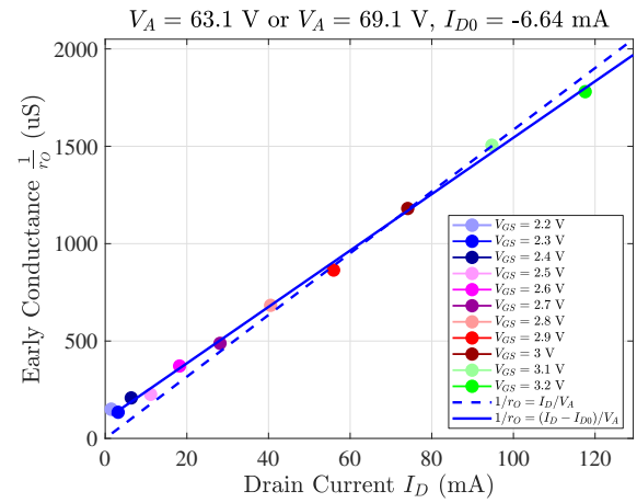
Figure 4.30: Early Conductance \frac{1}{r_O} vs. I_D
