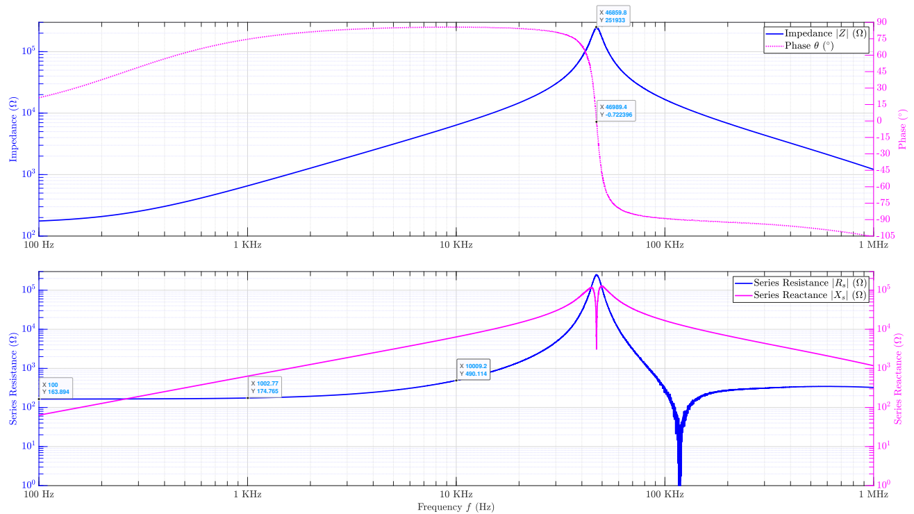
Figure 2.5: Impedance characteristics of the 100 mH DR magnetic core inductor
