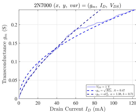
Figure 4.29: Transconductance g_m vs. I_D
