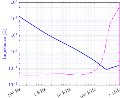
Figure 3.19: The capacitor's equivalent capacitance (left) and impedance characteristics (middle and right)
