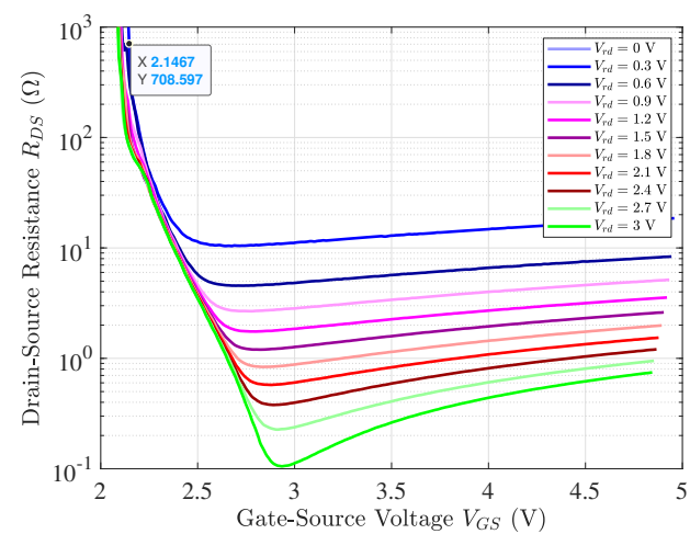
Figure 4.41: Drain-source on-state resistance
