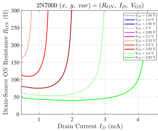
Figure 4.16: DS On-Resistance R_{DS(on)} vs. I_D
