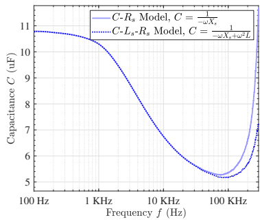
Figure 3.19: The capacitor's equivalent capacitance (left) and impedance characteristics (middle and right)
