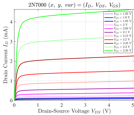
Figure 4.15: Static Characteristics I_D vs. V_{DS}
