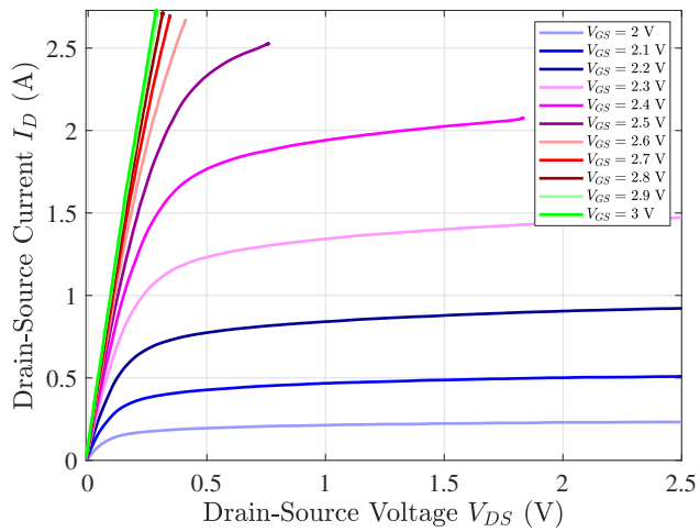
Figure 4.34: Output characteristics
