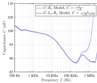
Figure 3.17: The capacitor's equivalent capacitance (left) and impedance characteristics (middle and right)
