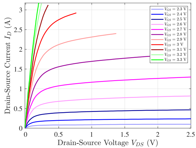
Figure 4.39: Output characteristics
