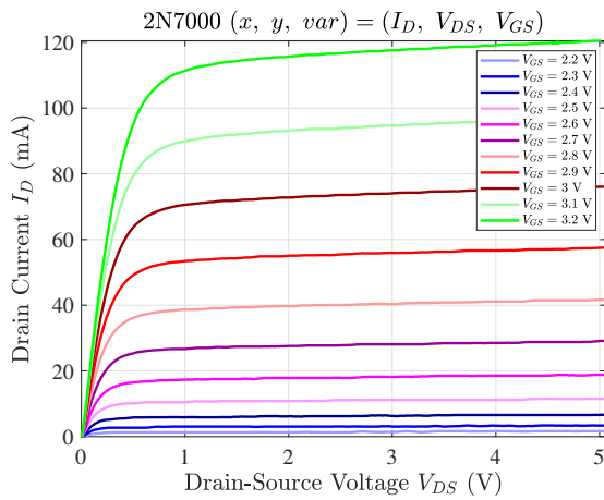
Figure 4.27: Static Characteristics I_D vs. V_{DS}
