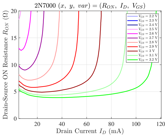
Figure 4.28: DS On-Resistance R_{DS(on)} vs. I_D
