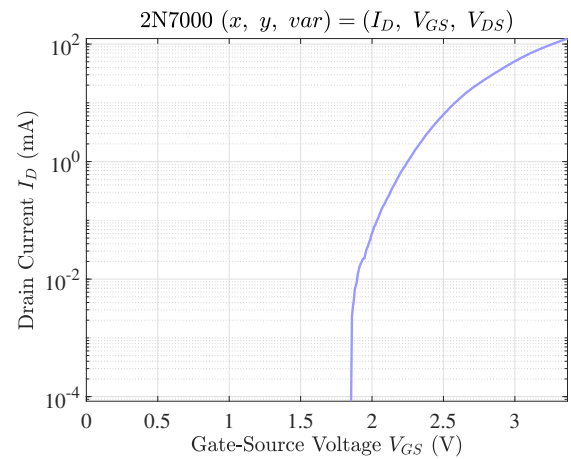
Figure 4.31: Transfer Characteristics I_D vs. V_{GS}
