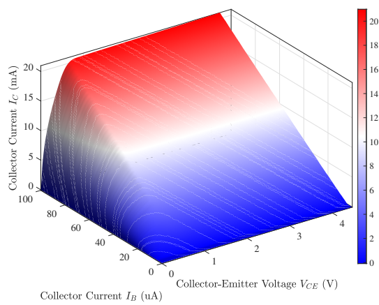
Figure 4.3: Static characteristics (low I_C and I_B , 3D view)
