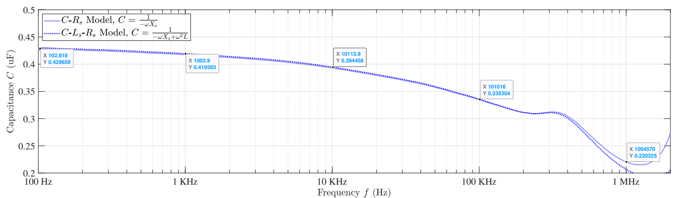
Figure 3.3: Construct the equivalent models
