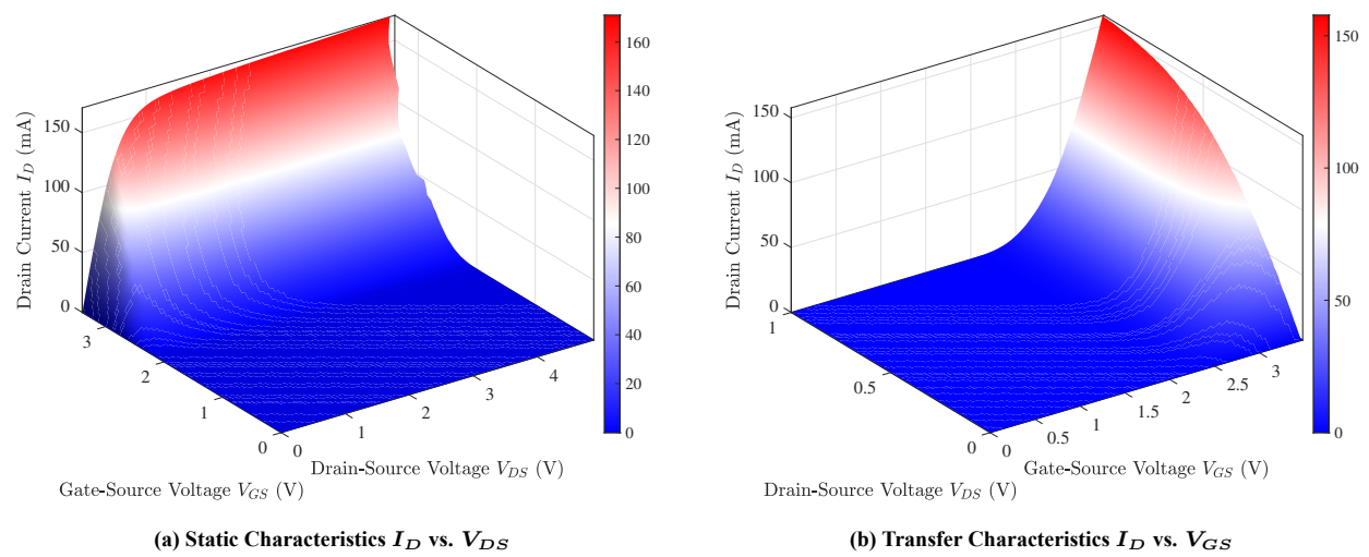
Figure 4.14: Characteristics of 2N7000 (3D view)
