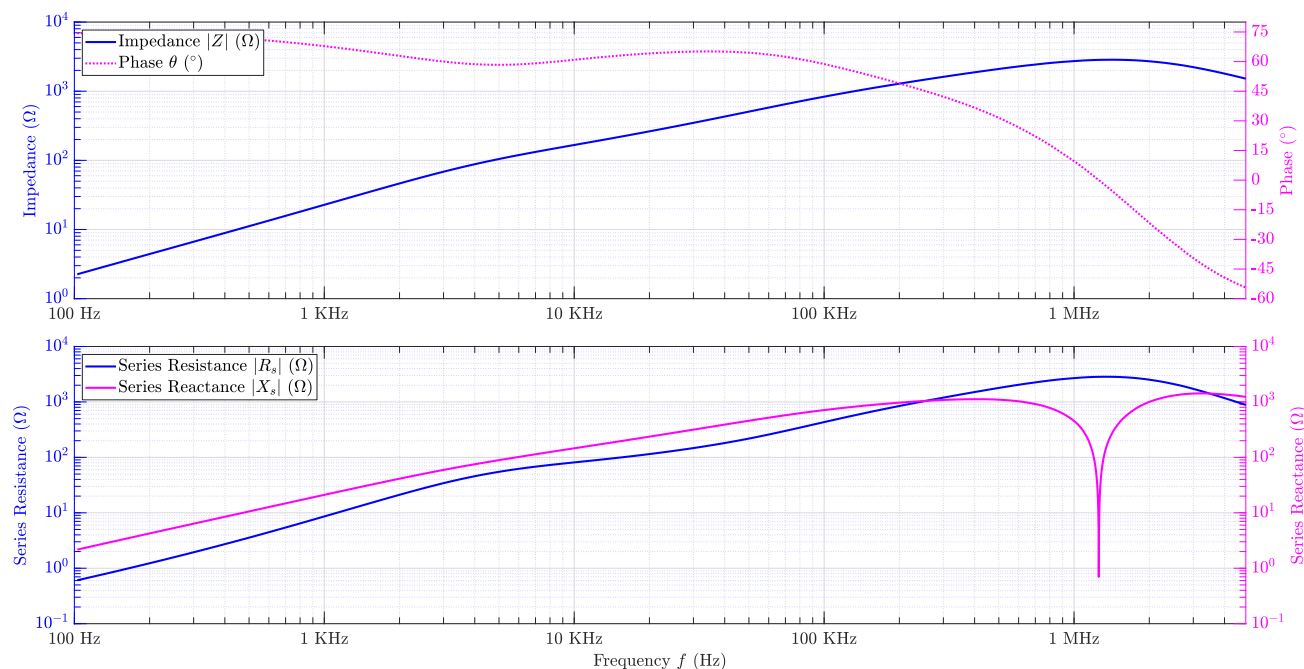
Figure 2.18: Impedance characteristics
