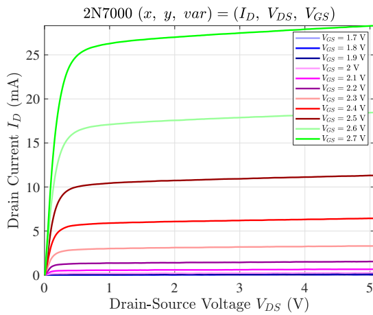
Figure 4.21: Static Characteristics I_D vs. V_{DS}
