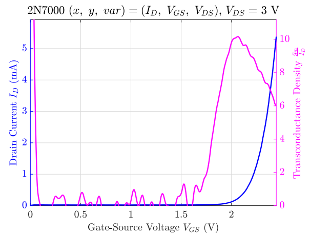
Figure 4.19: Transfer Characteristics I_D vs. V_{GS}
