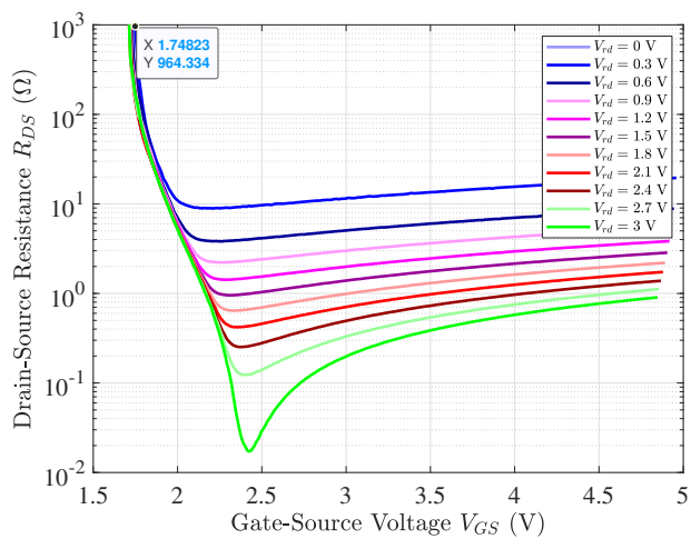
Figure 4.36: Drain-source on-state resistance
